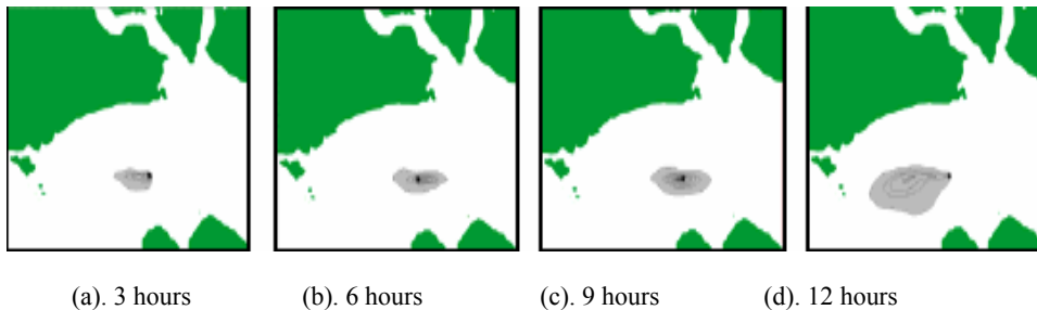
Figure 1. Dynamics of plume at the sea surface at different instances after the spill. The near-bottom source is located at the point marked by “*”.
